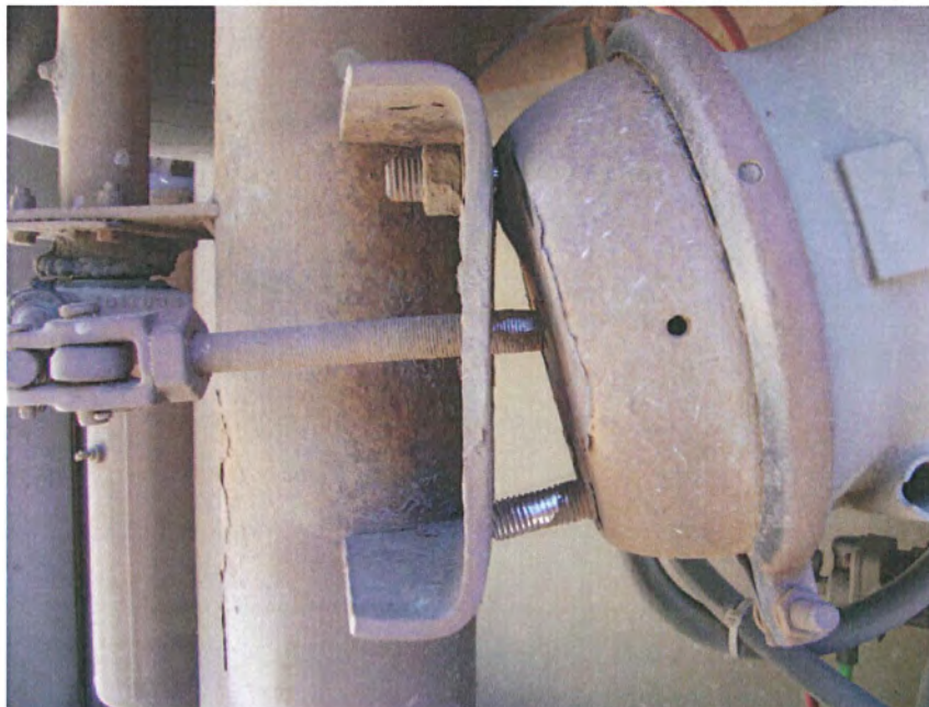
Photo # 10 – axle #9 loose brake chamber mount
