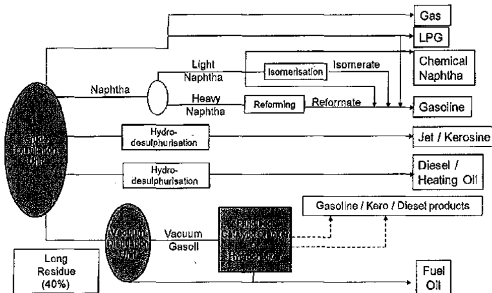
Figure 1: Key Processes in a 'Conversion' Refinery
