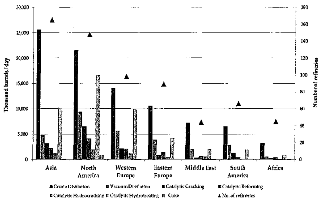
Figure 3: Global Refinery Capacity and Configuration
